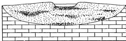
FIG. 10. Diagram showing general structure of strata deposits.
